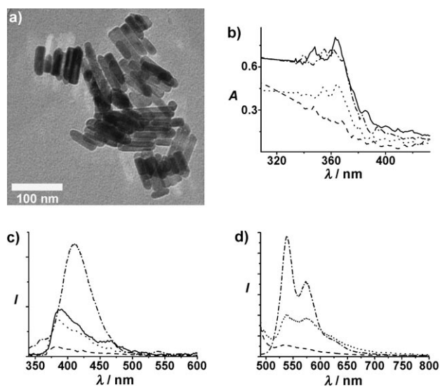
Figure 2. a) TEM image of ZnO NRs. b) The absorption spectra of PDI (---), ZnO NRs (—), ZPDI (----), and ZPDI with perylene (---) in DMF solution. The fluorescence spectra of PDI, ZnO NRs, ZPDI and ZPDI with perylene in DMF solution, c) \lambda_{\text{ex}} = 325 nm, and d) \lambda_{\text{ex}} = 475 nm.
