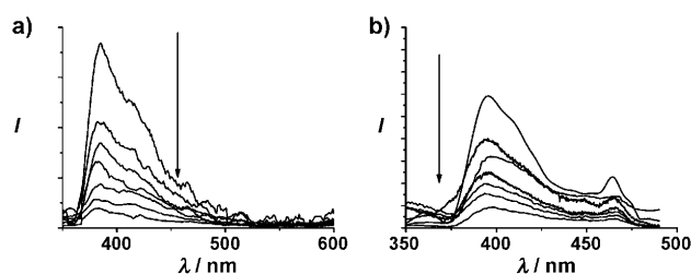
Figure 4. a) Fluorescence response of ZPDI to the addition of various concentration of perylene. b) Fluorescence response of ZPDIS after the addition of various concentrations of perylene. For (a) and (b), curves correspond to ZPDI or ZPDIS alone (highest intensity), and addition of 10^{-12} , 10^{-10} , 10^{-9} , 10^{-8} , 10^{-7} , 10^{-6} , 10^{-5} M perylene (lowest intensity), respectively. \lambda_{\text{ex}} = 325 nm.
