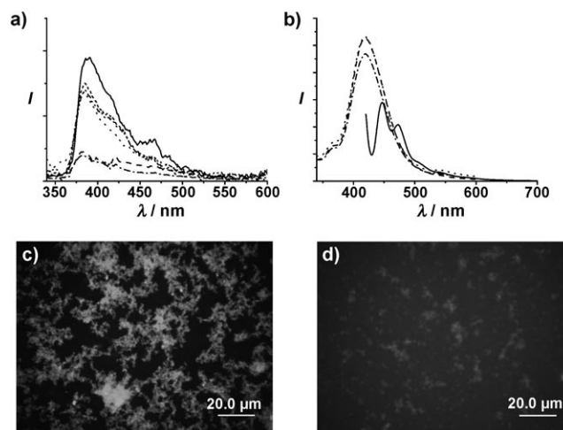
Figure 3. Emission spectra of a) ZnO NRs (—), ZPDI (.....), and ZPDI with perylene (---), anthracene (----), pyrene (---), and a PAH mixture (---). \lambda_{\text{ex}} = 325 nm; b) colloids of ZPDI with pyrene (---, \lambda_{\text{ex}} = 325 nm), anthracene (----, \lambda_{\text{ex}} = 325 nm), and PAH mixtures (---, \lambda_{\text{ex}} = 325 nm; —, \lambda_{\text{ex}} = 412 nm) in DMF solution after addition to 1 M aqueous hydrochloric acid. Confocal microscopy images of c) ZPDI and d) ZPDI with perylene ( 10^{-6} M; \lambda_{\text{ex}} = 470 nm).
